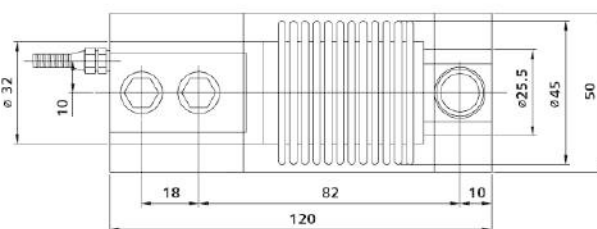
额定载荷(t) Rated Load D M 5,10,20,30,40,50,75 100,150,200,250 φ8 M8 300,500 φ10 M10
